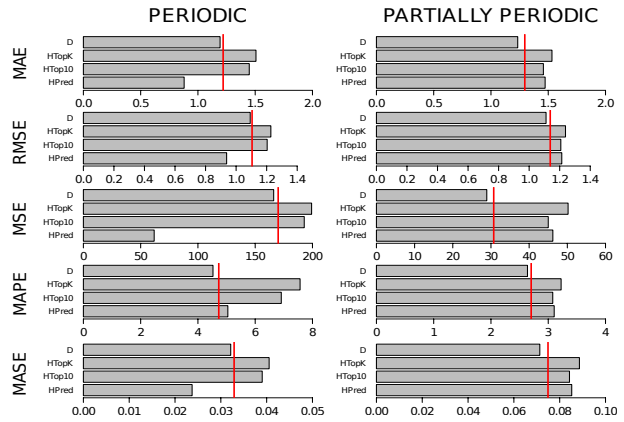
Figure 3: Evaluation of the hybrid model.
